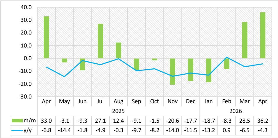
Chart 5: Beds Occupancy Index, Percentage Change
